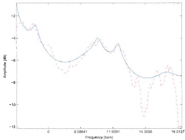
Figure 6.6: All-pole model fit (solid line) to the discrete, warped magnitude spectrum (dashed line).
