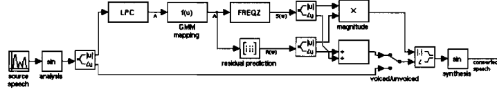
Figure 7.2: Block diagram of the HRT system.
