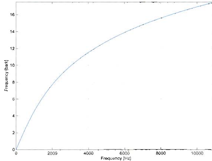
Figure 6.2: Frequency conversion between linear and bark scale
