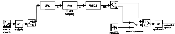
Figure 6.1: Block diagram for the spectral envelope transformation (SET) system.
