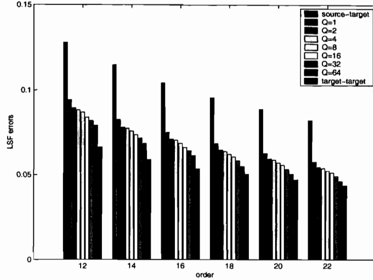
Figure 6.15: Inter-speaker, transformation, and target intra-speaker LSF training errors for the speaker combination M1→F2.
