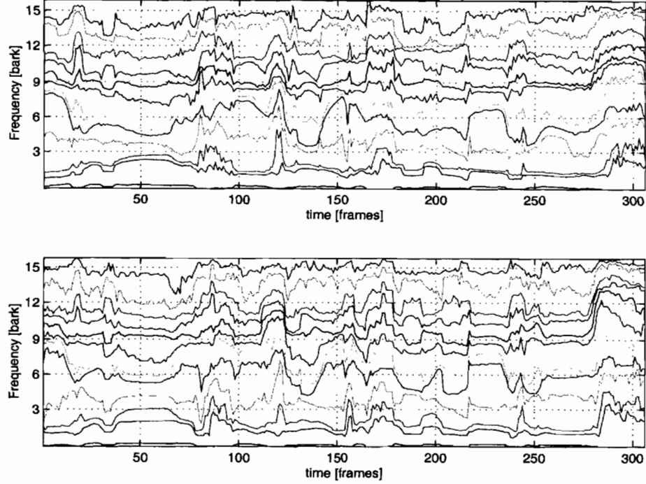
Figure 6.10: Two aligned LSF feature streams.
