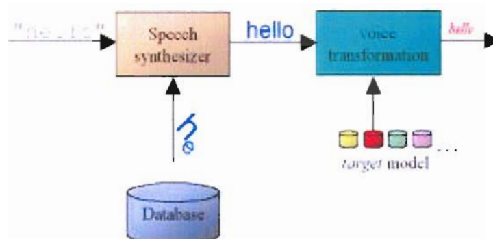
Figure 1.1: A text-to-speech synthesizer in conjunction with a voice transformation system. Fonts are used to represent speaker identity. The synthesizer retrieves chunks of speech from a database, according to an input text. The assembled synthetic speech is input to the voice transformation system, which uses a speaker model to render the final output speech to sound like a desired target speaker.
