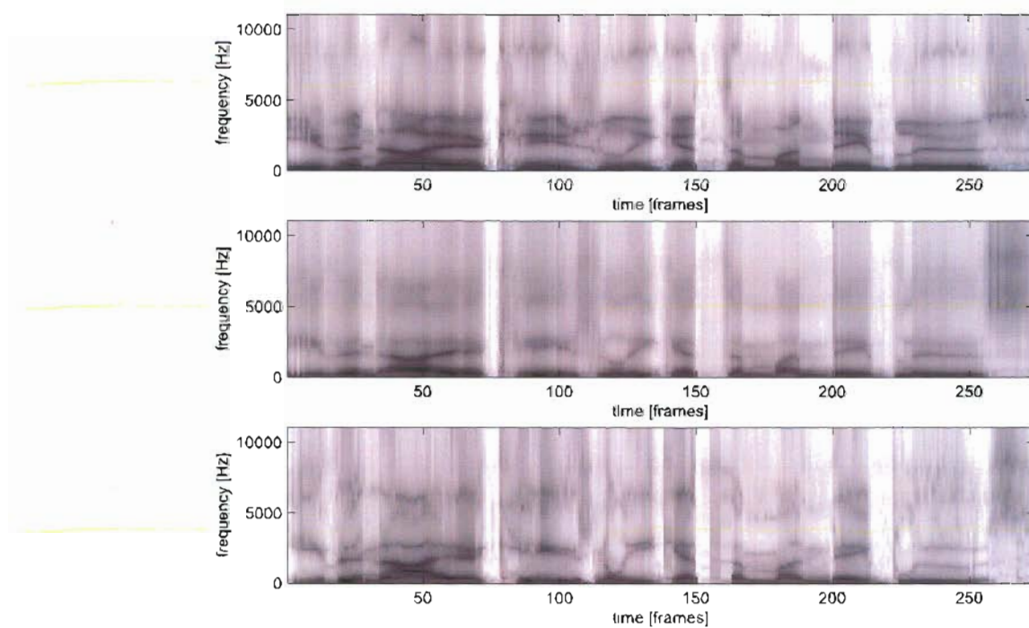
Figure 6.13: Unwarped, LPC log-magnitude spectrograms of the sentence “even I occasionally get the Monday blues”, derived from the source (top panel), transformed (middle panel), and target speaker (bottom panel).
