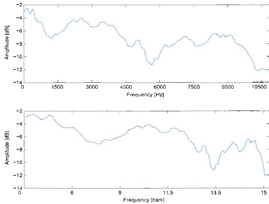
Figure 6.5: Sinusoidal magnitude spectrum before (top panel) and after bark warping (bottom panel).
