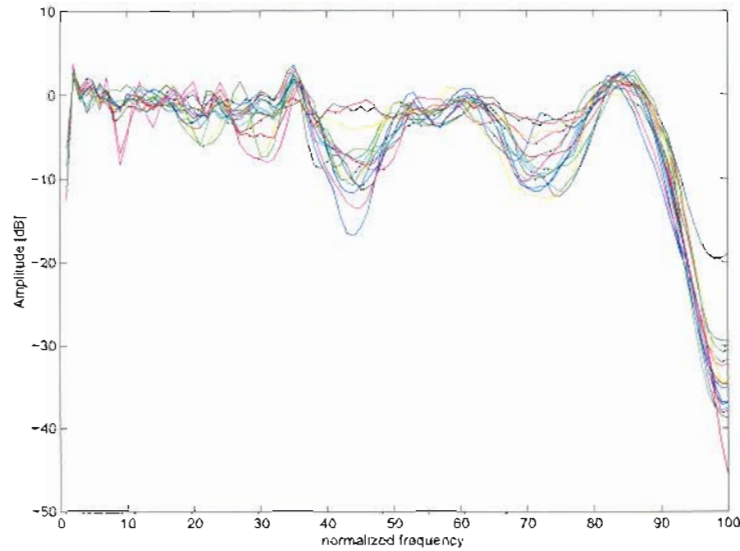
Figure 7.1: Magnitude spectra in a 16-entry residual codebook.
