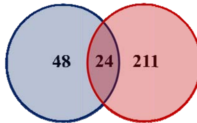
Figure 6: A) Count of DE genes from two gene expression datasets used in this study. Red indicates count of up-regulated genes and green indicates count of down regulated genes B) Overlap of biological processes between two gene expression data set
