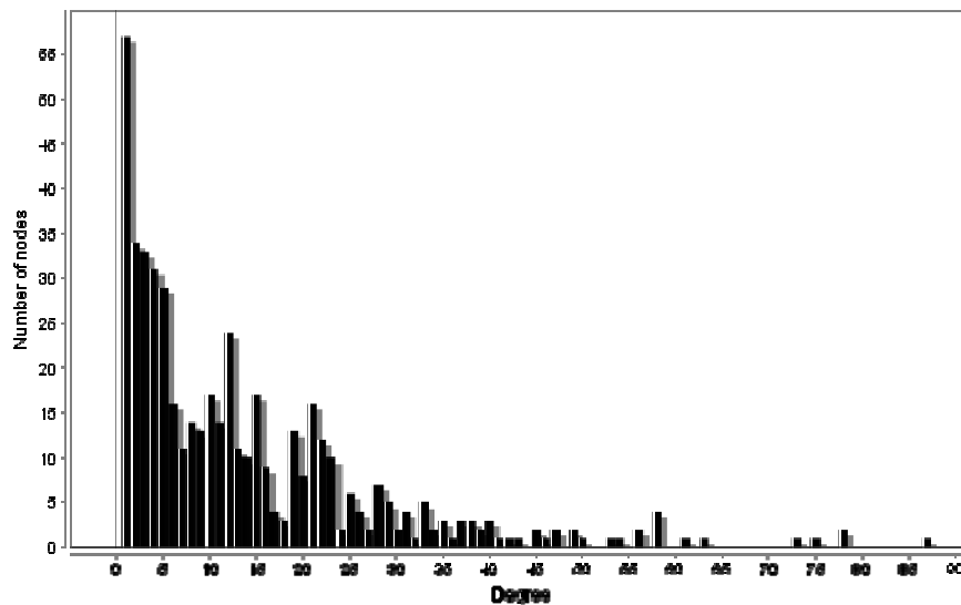
Figure 5 : Histogram representing distribution of degree (connected neighbors) of genes in the PPI network.
