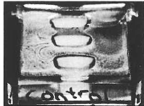
Figure 8: Vertically mounted specimens for KHN testing
