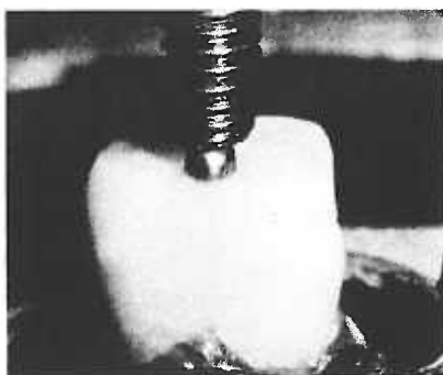
Figure 11: Fatigue cycler
