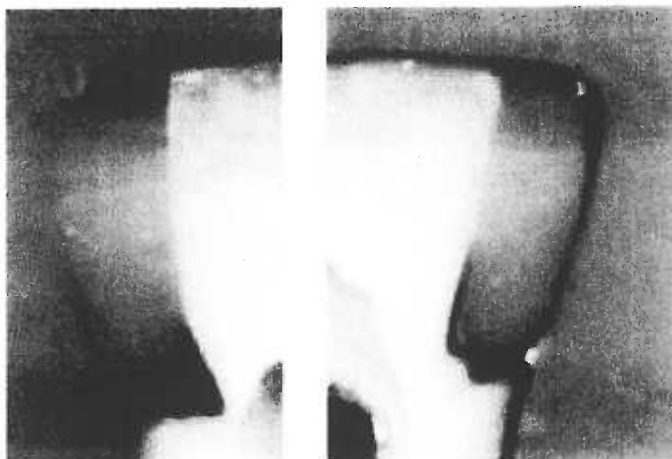
Figure 21: Microleakage: (l) pre-op; (r) 500K cycles 4000 \text{ mJ/cm}^2
